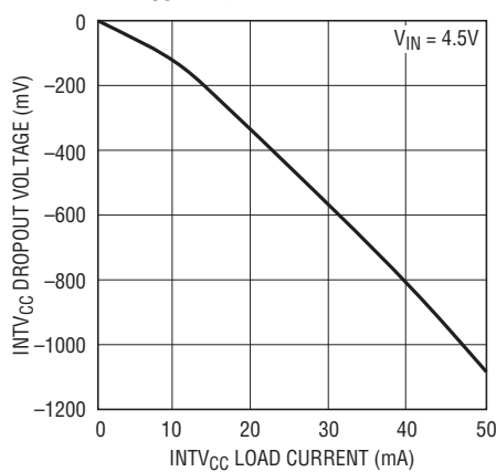
\text{INTV}_{\text{CC}} Dropout
